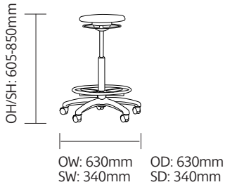
MSGL04 - Round Draughtsman PU Seat Weight: 7.7kg
