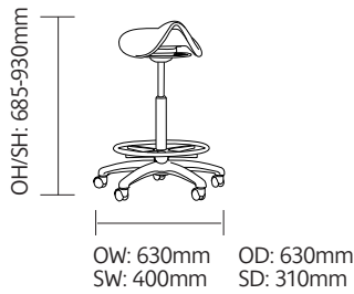
MSGL08 - Saddle Draughtsman PU Seat Weight: 10kg
