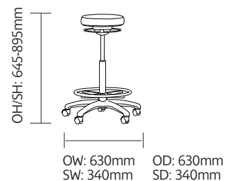
MSGL03 - Round Draughtsman Upholstered Seat
