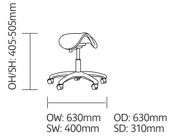
MSGL06 - Saddle stool PU Seat Weight: 8.8kg
