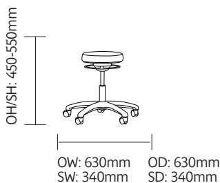
MSGL01 - Round stool Upholstered Seat
