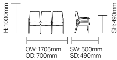
RSTL-ASSSA 3 Seater Beam with End Arms
