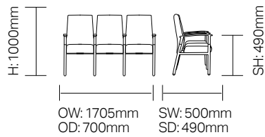
RSTL-ASASASA 3 Seater Beam with Intermediate Arms & End Arms
