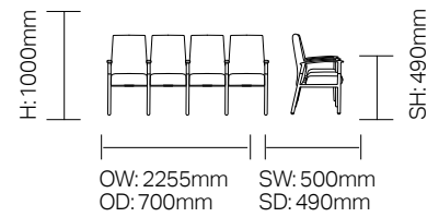
RSTL-4SEIA 4 Seater Beam with Intermediate Arms & End Arms
