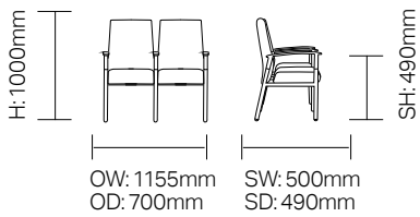
RSTL-ASASA 2 Seater Beam with Intermediate Arms & End Arms
