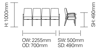
RSTL-ASSSSA 4 Seater Beam with End Arms
