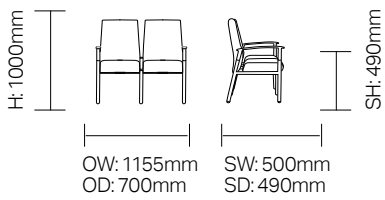
RSTL-ASSA 2 Seater Beam with End Arms
