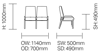
RSTL-SS 2 Seater Beam
