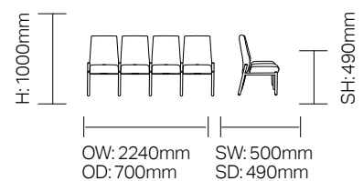
RSTL-SSSS 4 Seater Beam
